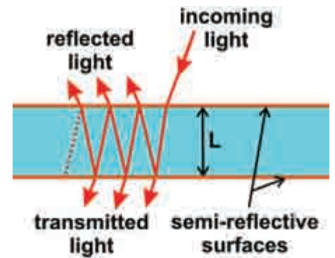
Image 6 – The Etalon, simply two parallel semi-reflective surfaces. Wave interference of the internal reflections allows only a particular wavelength to pass through. The distance between surfaces adjusts the pass band's centre wavelength, the reflectivity of the surfaces adjusts the pass band's width.
