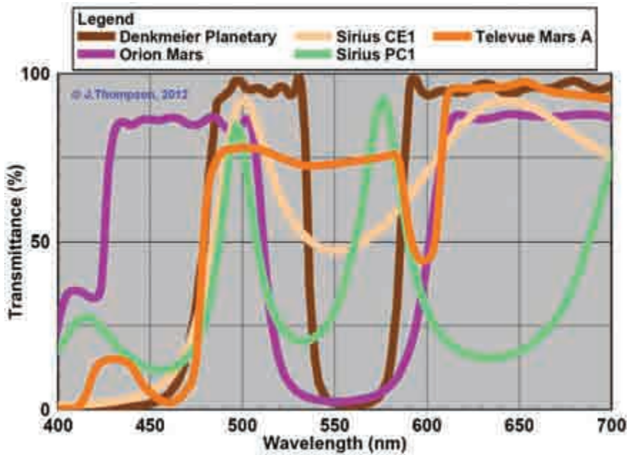
Image 2 – Spectral Response of Special Planetary Filters. Interference coating technology has been used to make filters that improve the contrast of planetary surface features.
