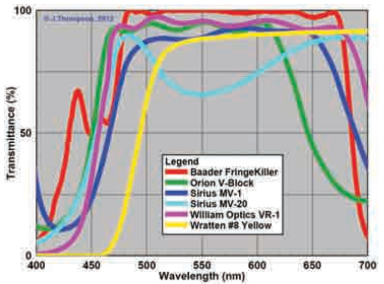
Image 4 – Spectral Response of Correction Filters. This group of filters is meant for removing the violet-blue end of the spectrum, greatly reducing the appearance of chromatic aberration in achromatic refractors.
