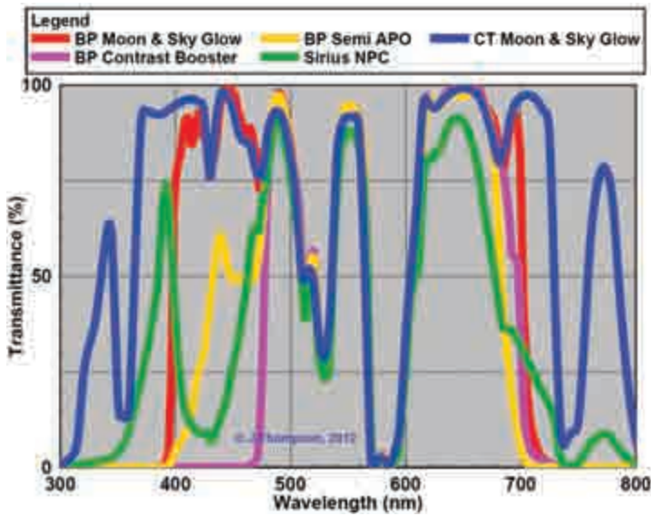
Image 3 – Spectral Response of Neodymium Filters. By infusing the filter glass media with the rare earth element neodymium, a unique and useful family of filters was created.
