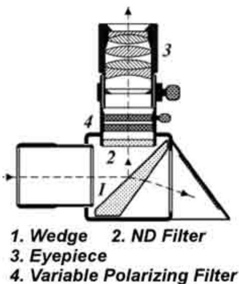
Image 5 – The Herschel Wedge. John Herschel first proposed the idea of using a wedge to split off a safe amount of sunlight for observation (left). His resulting observation sketches are as impressive today as they were 150 years ago (right).
