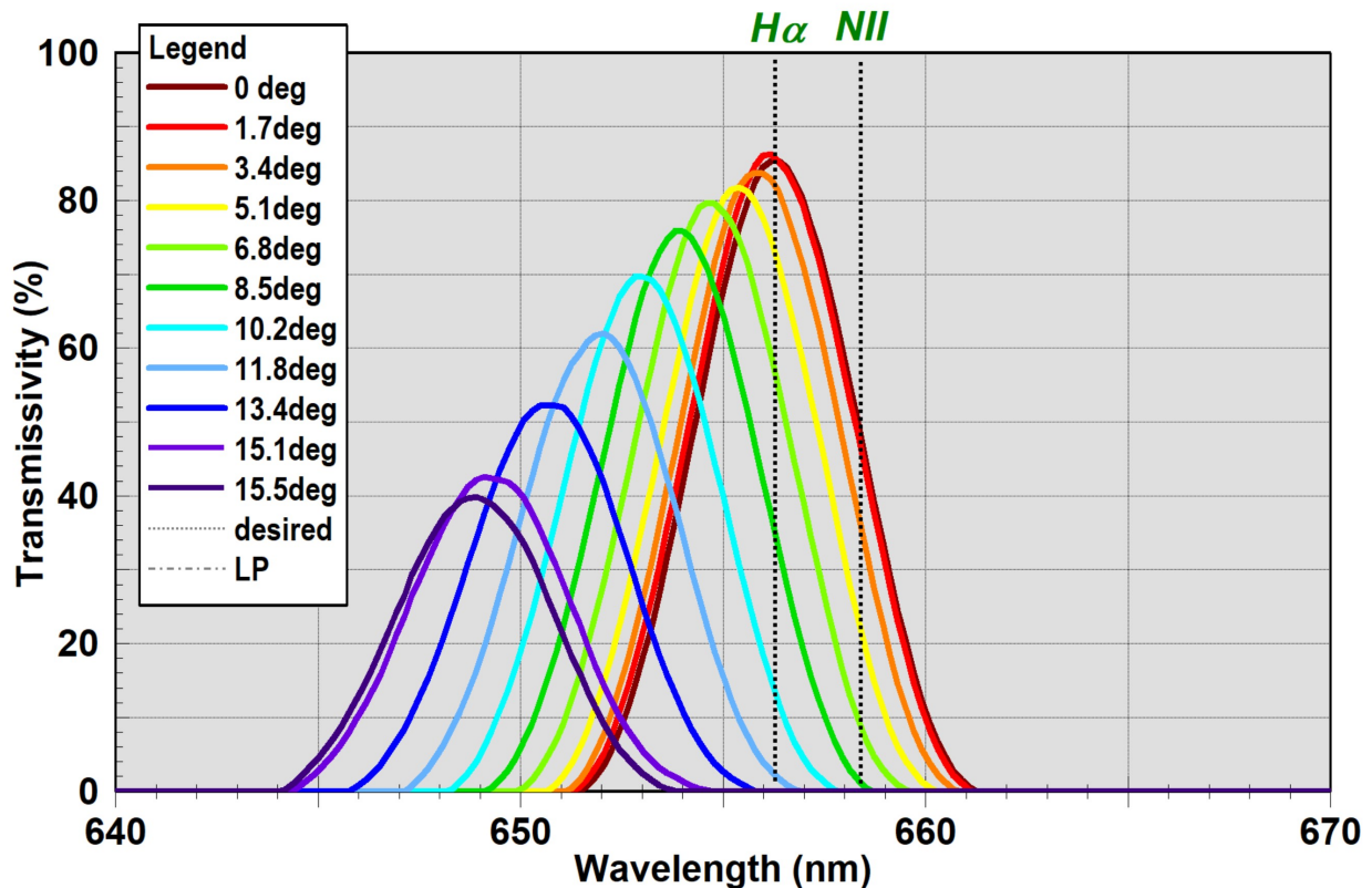
Figure 2 Measured Spectral Response of Radian Triad Filter vs Angle – H-alpha Band
