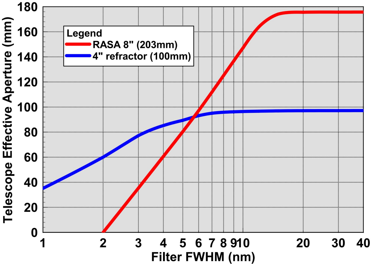
Figure 5 Predicted Scope Effective Aperture vs Filter FWHM
