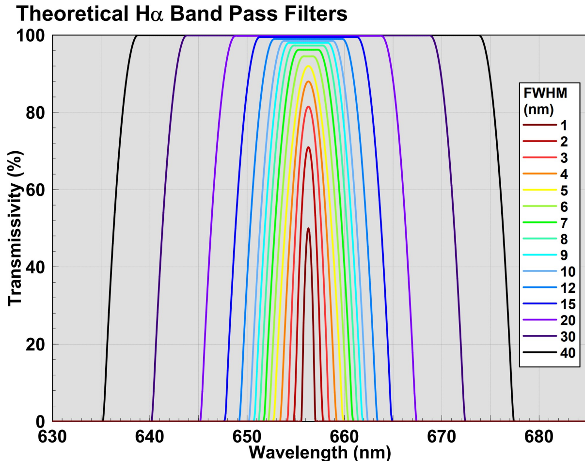
Figure 1 Spectral Response of Generic H-alpha Narrowband Filters
