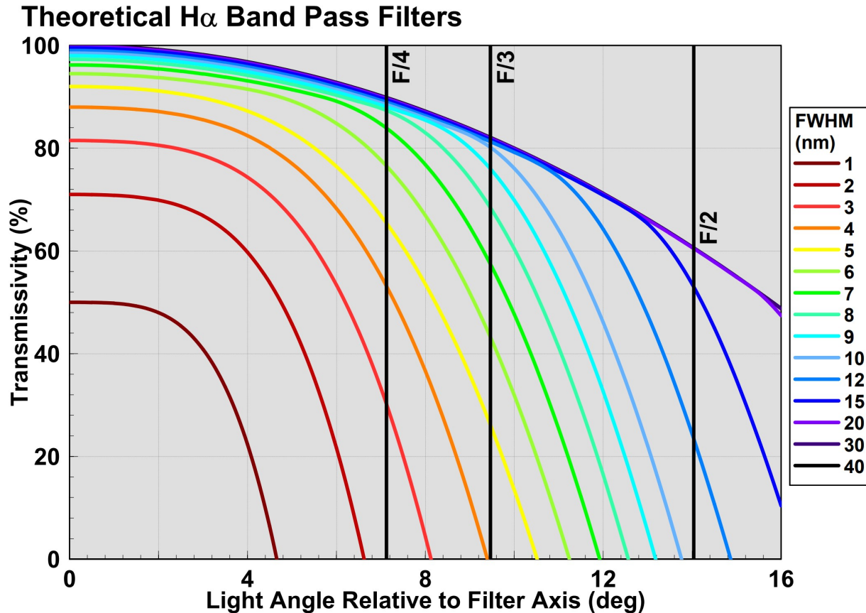
Figure 4 Predicted Generic Filter H-alpha Transmission vs Angle
