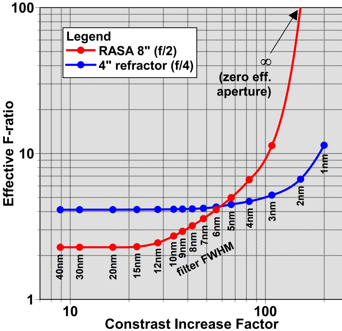
Figure 6 Predicted Scope Effective F-ratio vs Filter Contrast Increase
