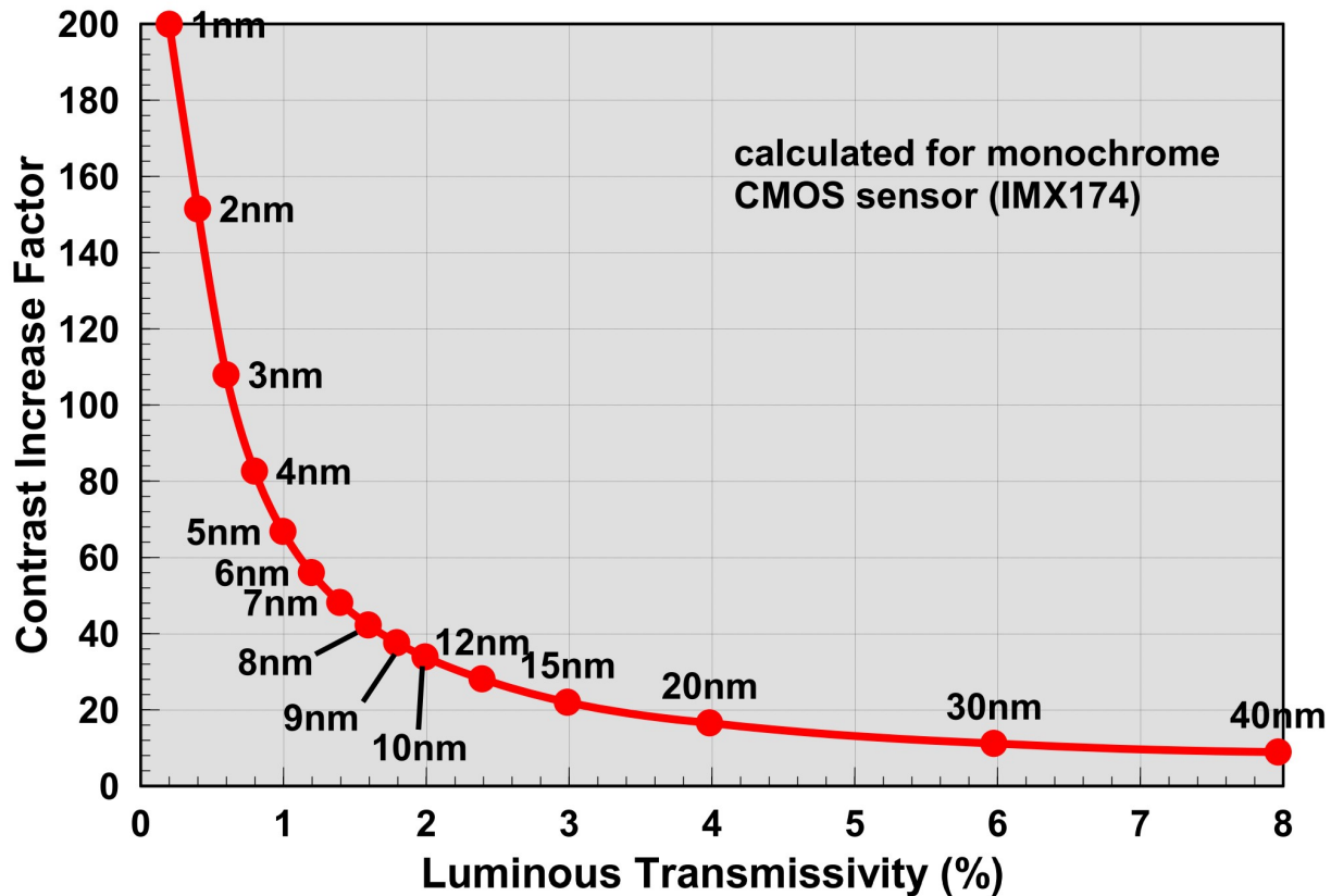
Figure 3 Predicted Generic H-alpha Filter Contrast Increase vs Luminous Transmissivity
